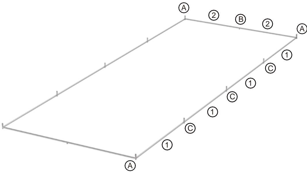
Tube 1 x8
