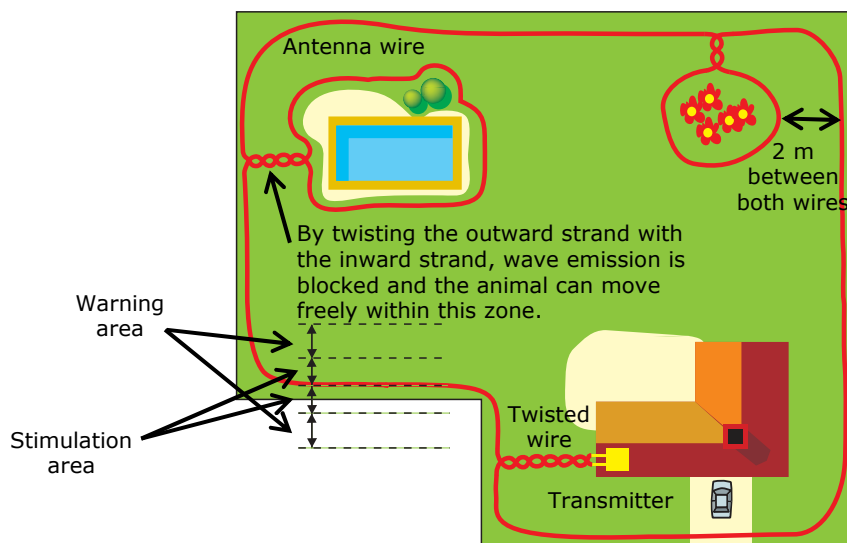
Diagram 4 – Sample installation
